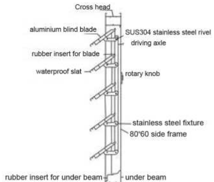
Manual aluminium blind (open to 45°)
