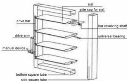
Manual aluminium wing blind
