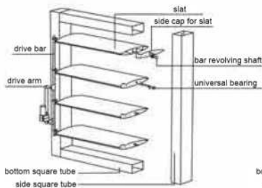
Motorised aluminium wing blind
