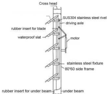
Motorised aluminium blind
