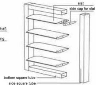
Fixing aluminium wing blind
